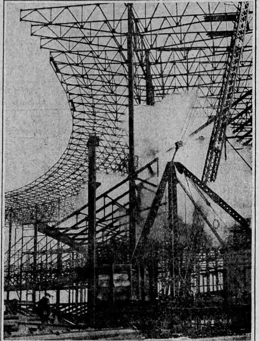
THE STEEL TAKING SHAPE in this striking photographic study represents the nucleus of a curve in Cleveland's great stadium which is being erected on the shores of Lake Erie at an expense of $2,500,000. When completed, it will have a seating capacity of 85,000, including 13,000 bleacher seats.
