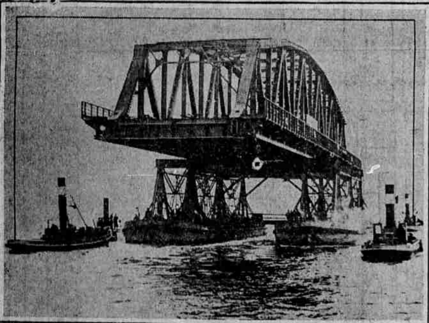
WHEN A BRIDGE GETS A LIFT —A sight rarely to be seen is one like that above, at Keizersveer, Holland, showing two freighters carrying a newly constructed bridge to its location. Of course, the tugboats helped out a bit.
