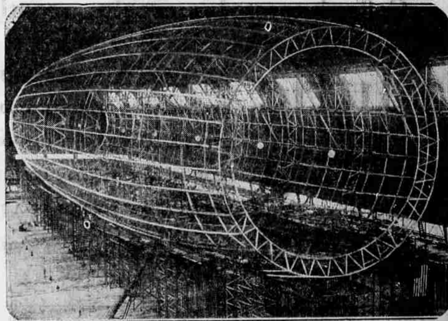
One of the navy's super-dirigibles, which when completed will be the largest ship of its kind in the world, is shown under construction at Akron, Ohio. This is the first of two dirigibles which will be built for the navy.
