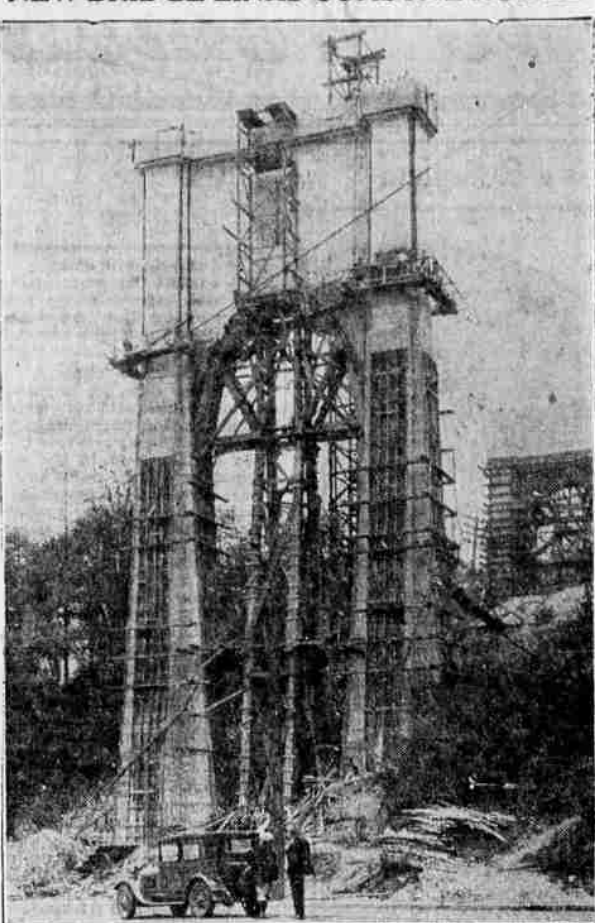
An approach pier of the $4,500,000 cantilever bridge in Seattle, Wash. which will be 2955 feet long and 165 feet high from water to roadway...
