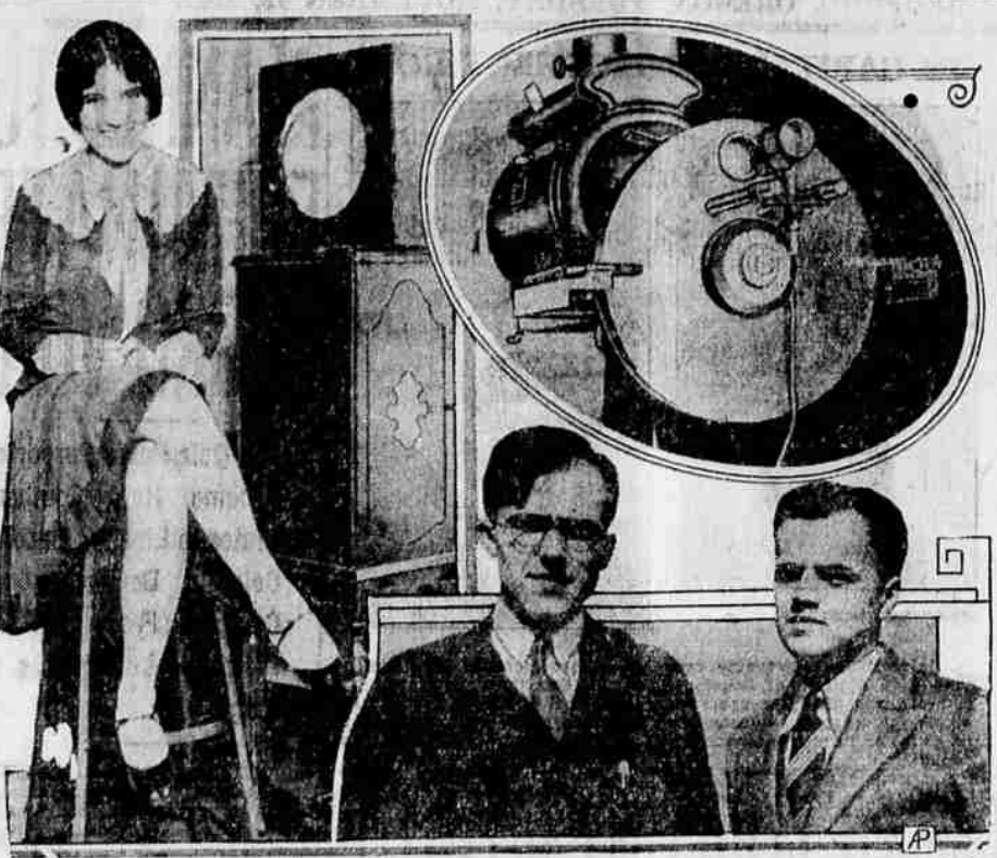
The men are Chicago engineers, Prof. L. Garner (left) and U. A. Sanabria, developers of a television system requiring only half the usual 100-kilocycle band. Above them is the new transmitter. The girl is Yvonne Metz, being televised by a portable 'electric eye' with a 12-inch photoelectric cell.
