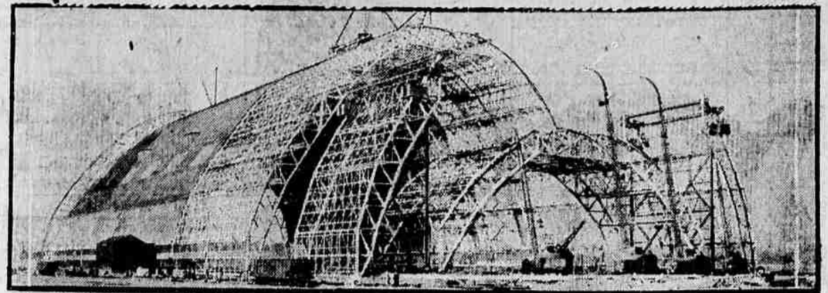
A STRIKING VIEW OF THE GOODYEAR ZEPPELIN HANGAR being built at Akron, O., for housing of the huge dirigibles to be built for the U. S. navy is pictured above. When complete, there will be 13 massive arches. This picture shows fabrication of one of the arches. Note the topmost part of the arch on the ground, with the sides already erected.
