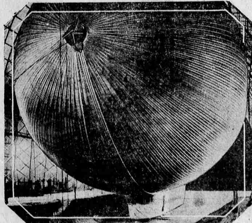
A STEAM-DRIVEN ALL-METAL DIRIGIBLE is next on the air program. This shows the nose of the huge ship nearing completion at its Glendale, Calif., hangar. The blower which creates a partial vacuum (the circular section exposed) makes an air pressure which drives the ship forward.
