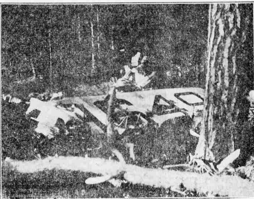
The wing of the ill-fated Transcontinental Air Transport's City of San Francisco, heading the mangled "snatch" which Lt. George H. Rice of the Western Air Express saw from the skies as he searched for the missing ship and enabled him to locate the wreck after seventy planes and hundreds of men had searched five days for it. The transport crashed on the rugged south slope of Mt. Taylor in New Mexico last Tuesday, killing its eight occupants. One of the stout pine trees such as the ship struck when it dove headlong into the mountainside, wrecking it, can be seen in the foreground.
