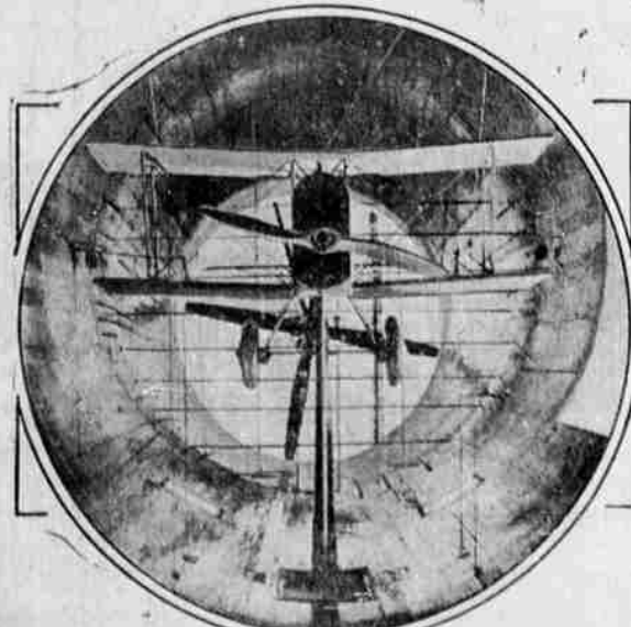
ARTIFICIAL GALES whiz through this tunnel at 90 miles an hour. It is part of the aeronautical laboratory at the Massachusetts Institute of Technology, and in it models of planes are suspended and every movement registered on delicate instruments.
