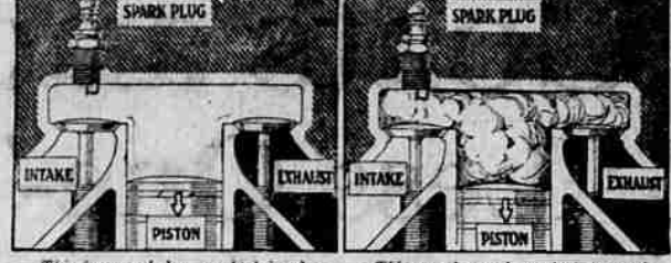
This hot spark has resulted in the cylinder mixture being entirely burned. Complete combustion shown by white. This weak spark produces a much slower burning combustion. It is not completed, as at the left. White shows unburned gas.
