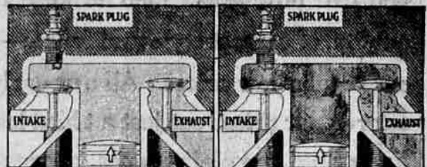
Here the burned gas is being forced out through the exhaust valve. Fuel power is shown, no live gas escaping. Here loss of power shown by slow burning. It is completed because live gas is actually being expelled through the exhaust.
