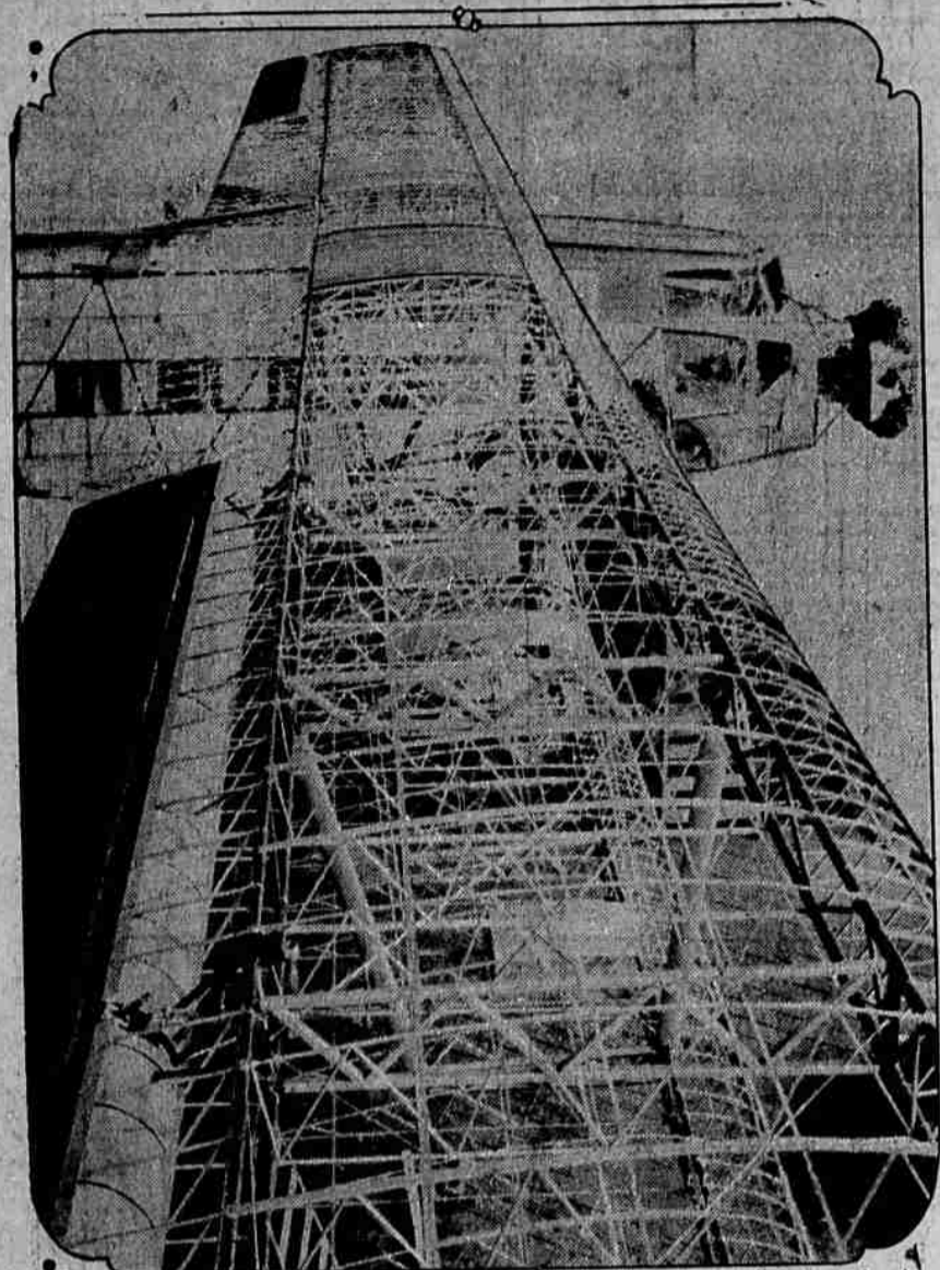
AN IDEA OF THE MAZE OF CONSTRUCTION necessary in an airplane wing is gained through this picture of the skeleton of one of the wings of a transcontinental tri-motored 18-passenger transport to be flown by the Boeing System between Chicago, Oakland and San Francisco. The plane has an 80-foot wing span.
