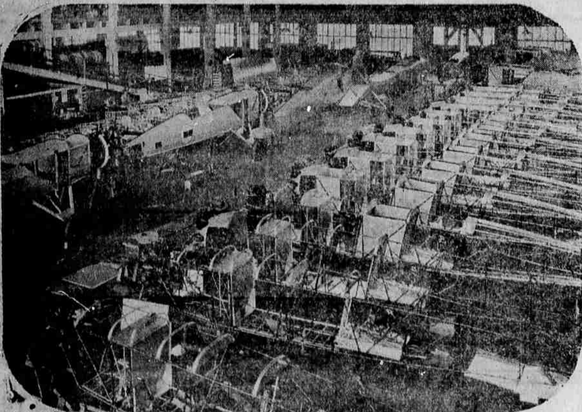
THE MANUFACTURE OF AIRPLANES IS "BIG BUSINESS" NOW—and if you don't believe it, take a look at this picture, snapped in the assembly room of the Boeing Airplane Co.'s factory at Seattle. A fleet of the famous A-40 mail-passenger planes is shown nearing completion. When finished, these planes will fly on the transcontinental and Pacific coast air mail lines.
