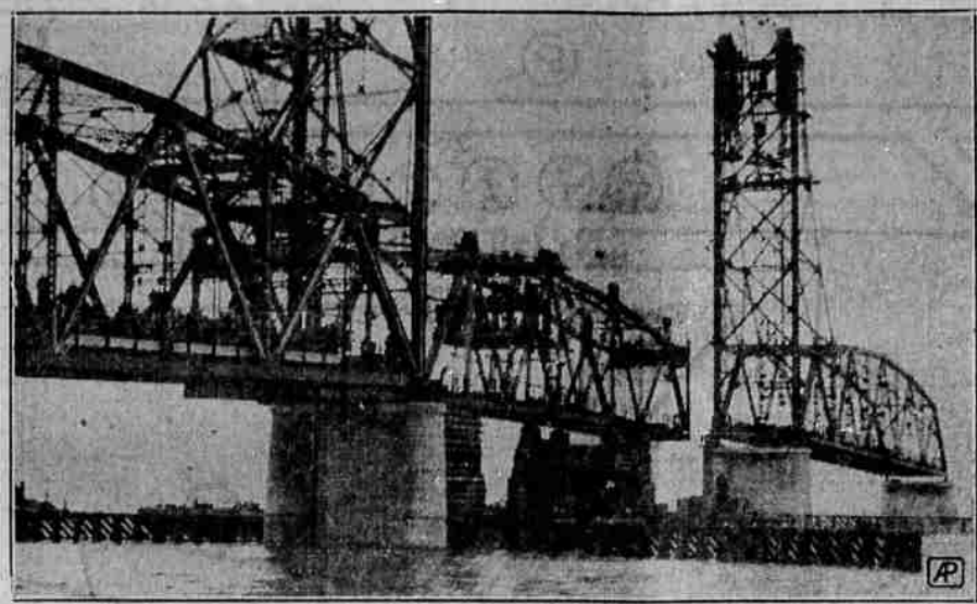
Towed ten miles, a 303 foot portion of the San Mateo bridge across San Francisco bay was fitted to adjoining spans as the tide went out. The structure is 7.1 miles long.
