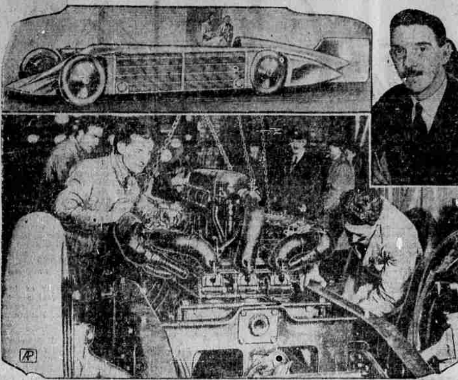
Engineers are shown assembling the 1,000 horse power "Golden Arrow" in which Major Segrave hopes to regain for England the world's automobile speed record at Daytona Beach, Fla. Upper left is how the automobile will appear when completed. At right is Capt. J. S. Irving, designer of the machine.
