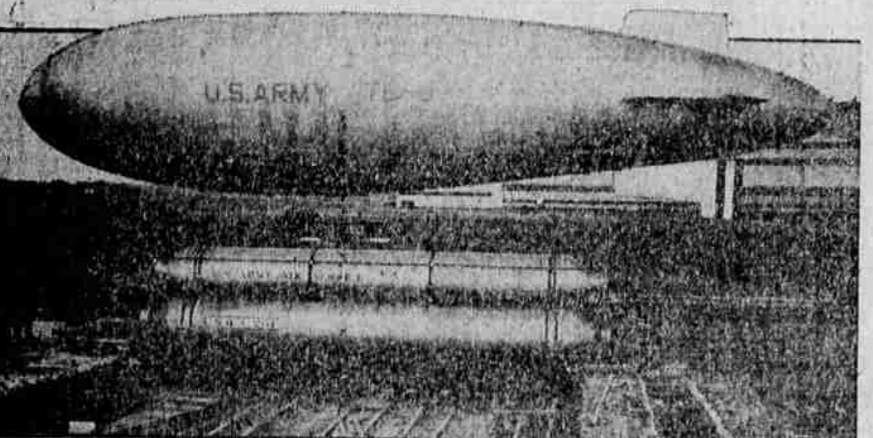
HELIUM GAS FOR UNCLE SAM'S BIG SILVER AIRSHIPS is now transported across the country in two new tank cars, especially designed for the purpose and owned by the army air corps. Three large cylinders, holding enough helium to inflate any army blimp, are on each car. This shows one of them, with the dirigible TC-8 in the background.
