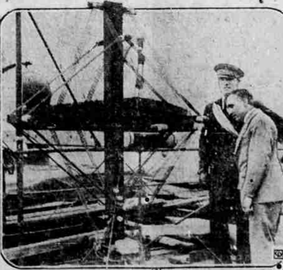
View of one of the radio masts being taken to Spitzbergen by General Umberto Nobile's North Pole expedition for communication with the remainder of the world during the flight. Photo shows the electrical officer of the expedition and a radio expert examining the mast.
