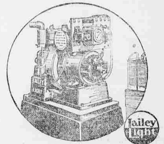
Lalley Light is a complete unit—engine and generator—with 16 cell storage battery. It supplies ample electricity for lights, water pump, washing machines, vacuum, cream separator, tanning mill, iron, etc.
