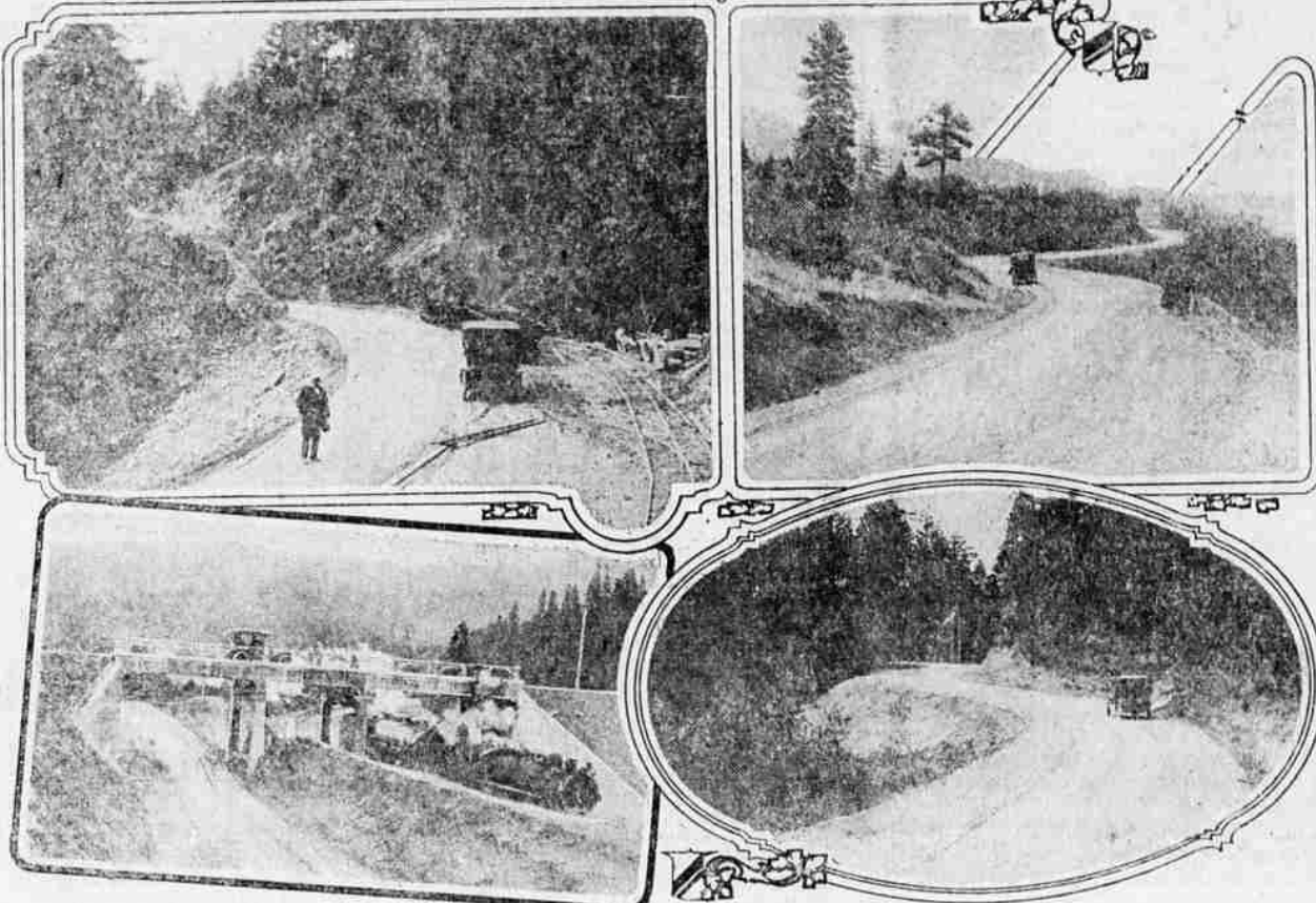
Top, left to right—Paving construction equipment; summit of Siskiyou six miles from California line. Bottom, left to right—Viaduct at Steinmann crossing, Southern Pacific; north slope of Siskiyou grade.
