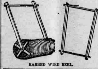
BARBED WIRE REEL.
