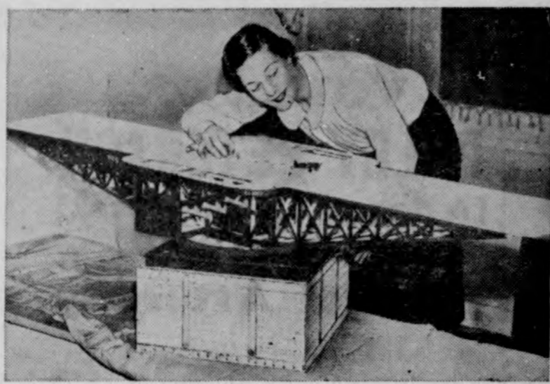
A model of a rotary elevated airport, designed by Captain Charles Frobisher was exhibited at the Inventions Exposition held recently in Central hall, London, England. One of the big advantages claimed for the rotary airport is that it can be turned in the direction the wind is blowing, thus facilitating the take-off and landing of planes.
