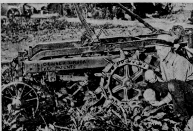
Of almost human ability at "topping" and digging sugar beets is the recent invention of John Devey, Jr., of Glendale, Calif., shown here with his device. Weighing 3,000 pounds, the machine in one operation slices the tops from the beets, and digs them from the ground 60 times as fast as the average worker.
