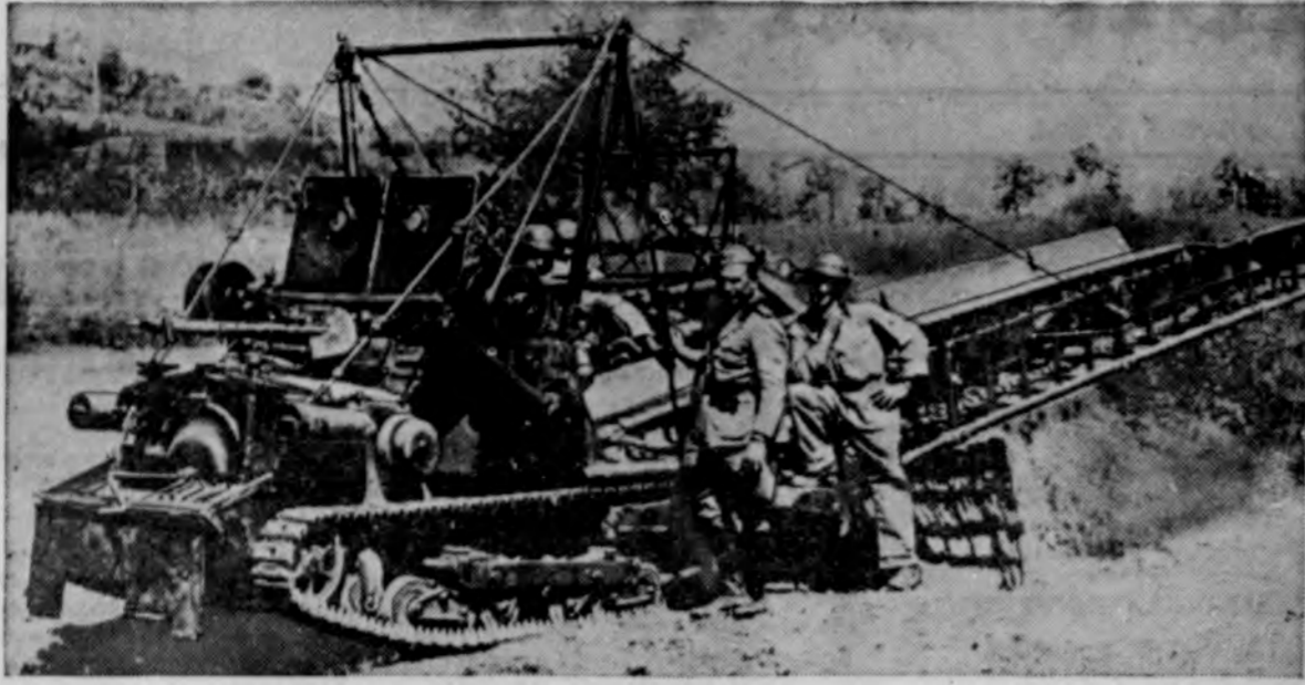
This is a new Italian tank which carries a bridge for transporting soldiers over small rivers. It was demonstrated for the first time at the huge Italian war maneuvers held near Avellino recently.
