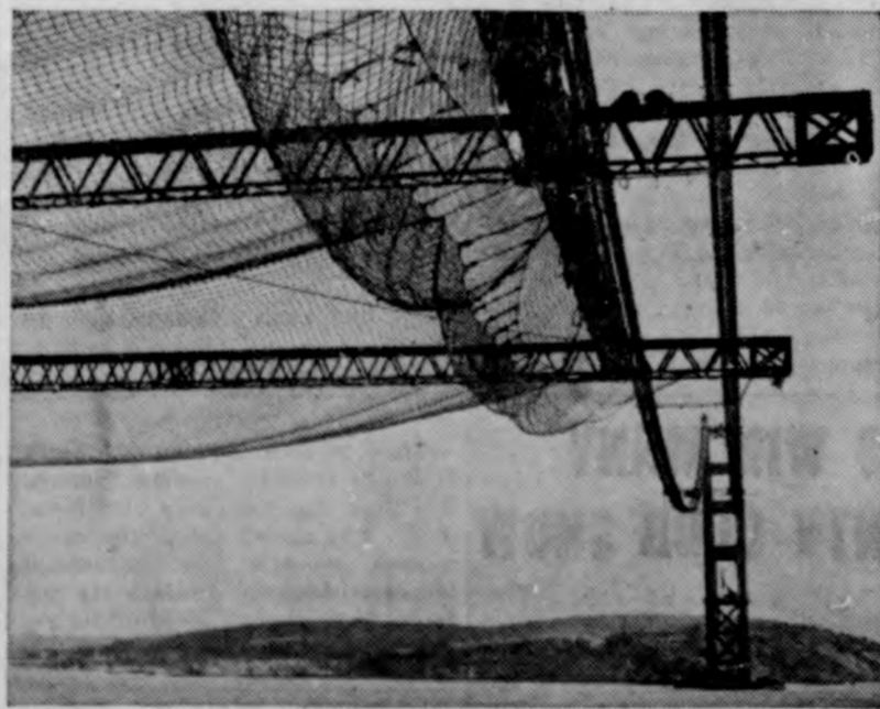
Pictured here is a section of the great net which has been swung beneath the Golden Gate bridge at San Francisco to insure its being "the safest job in the world." The net, first of its kind to be used in construction history, has been swung thirty feet below the bridge and is designed to prevent workmen plummeting to their death from the dizzy heights of the bridge in the event of a fall.
