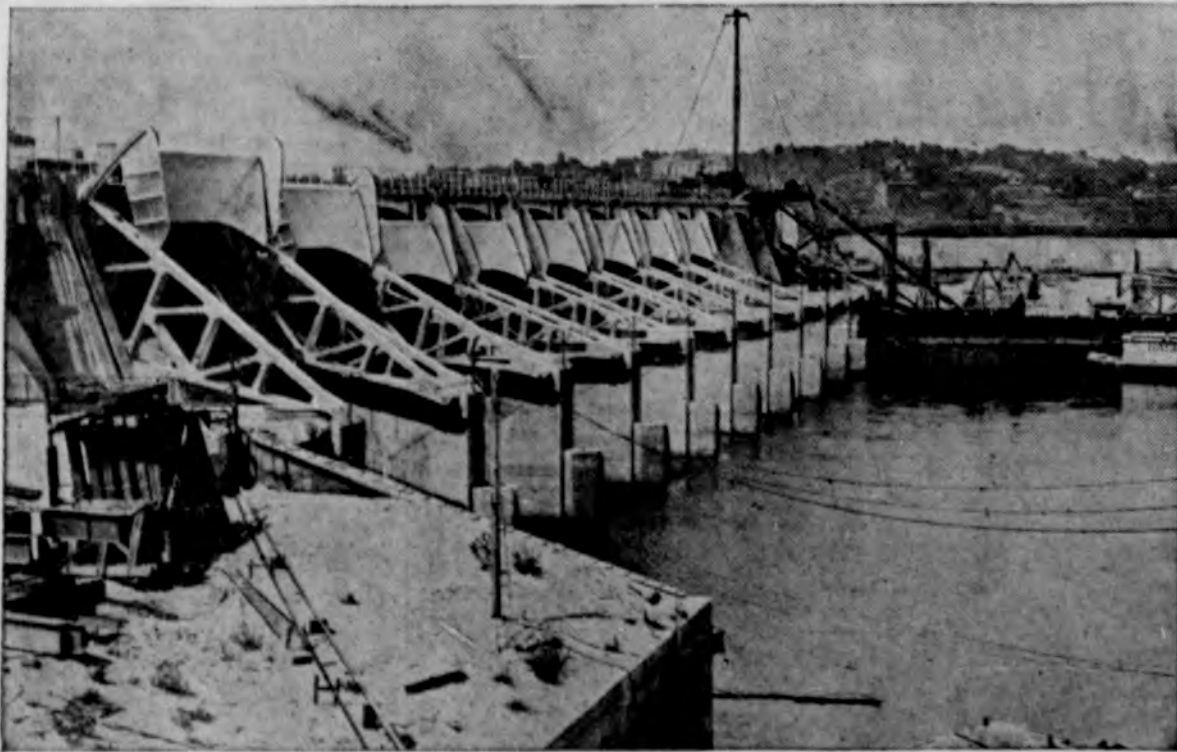
One-third of the great navigation dam across the Mississippi river at Alton, Ill., has been completed and work on the remaining section of this the longest and highest of the 26 dams projected to aid navigation on the Mississippi between here and St. Paul, Minn., is progressing swiftly. The dam's 30 gates will be the largest of their type in the world. The dam proper will be 1,724 feet long in addition to the width of an already completed lock on the Alton shore. View shows a general view of the dam project with the completed gates in the foreground and a coffer-dam in mid-stream, in which the second series of gates will be built.
