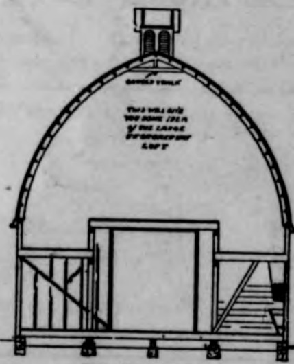
CIRCLE ROOF BARN
