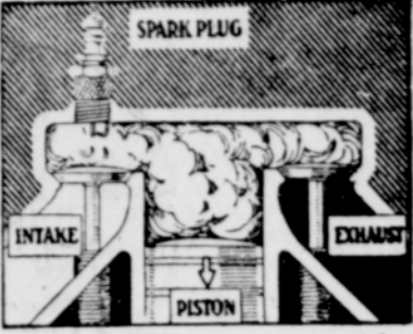
This weak spark produces so much slower burning that combustion is not completed, as at the left. White shows unburned gas.
