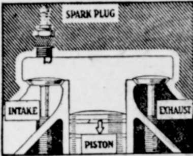
This hot spark has resulted in the cylinder mixture being entirely burned. Complete combustion shown by white.
