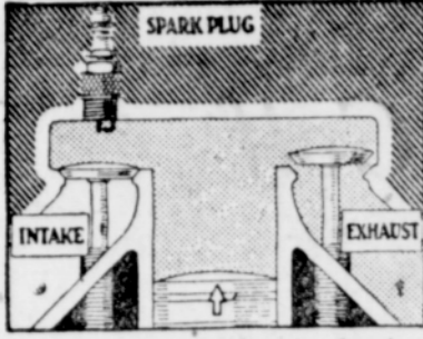
Here the burned gas is being forced out through the exhaust valve. Full power is shown, no live gases escaping.
