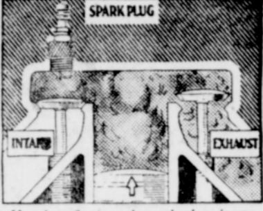
Here loss of power is shown by slow burning of the mixture. Live gases actually being expelled through the exhaust.
