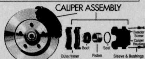
CALIPER ASSEMBLY
