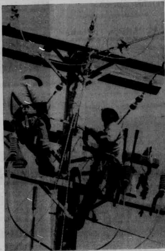
Vern Wilson and Ed Struthers, Columbia Basin employees, are making final ties into a hot line to serve Kinzua Corporation with a new 1,550 kva transformer which will serve the new plywood mill.
