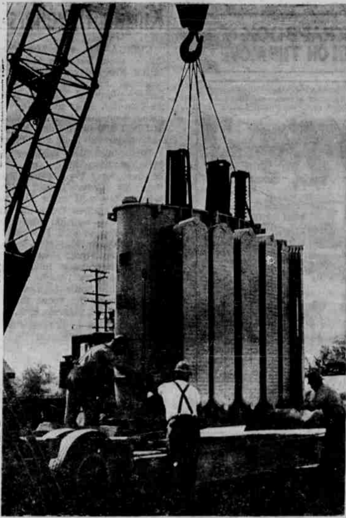
EASY DOES IT. Fifty thousand plus pounds of transformer settles down gently on the low boy for transportation to the site of the new Heppner Sub-station. Working on the transfer are Art Vance, Bud Marshall and Vernon Wilson.
