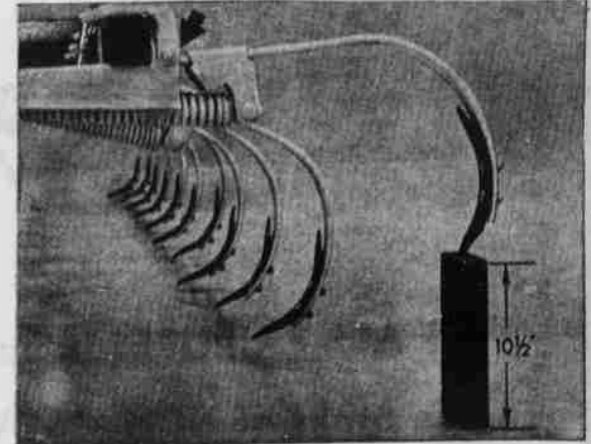
Unmatched for fore and aft clearance between ranks — Heavy trash, big rocks, and other debris have plenty of room to get through the wide rank spacings on all models, making them unusually hard to clog.
