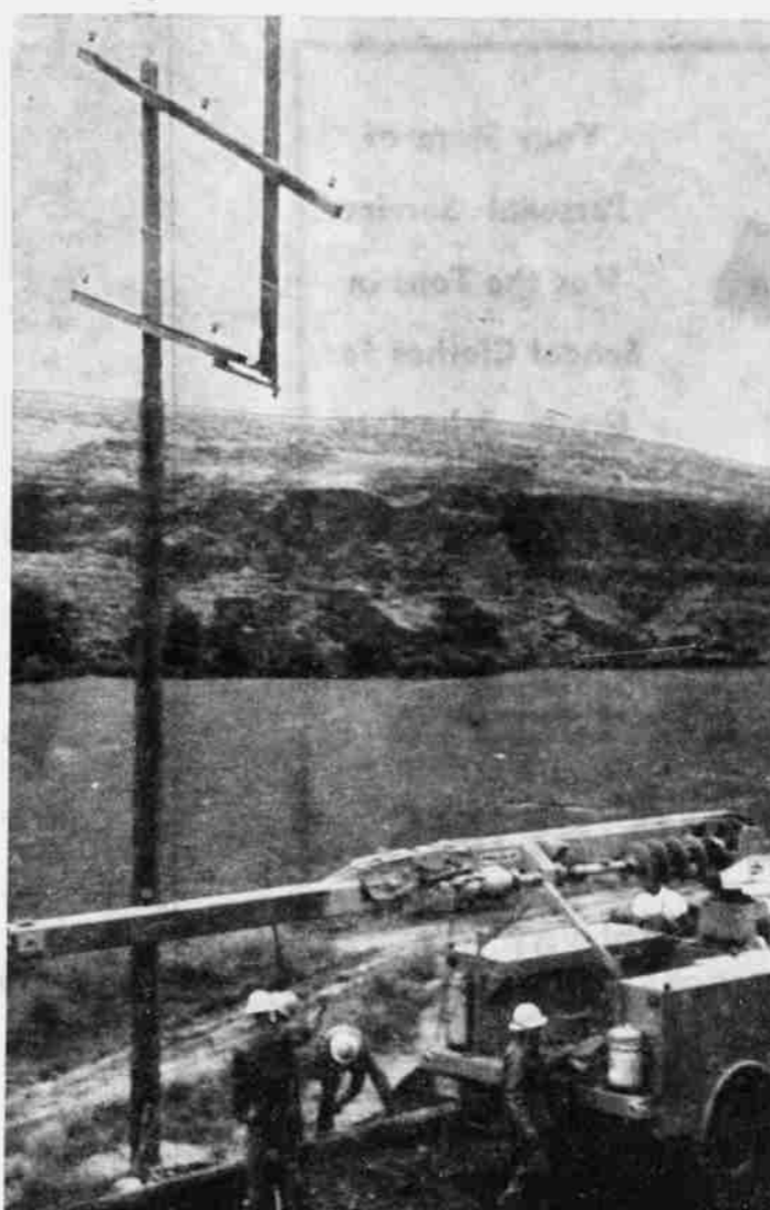
This picture shows damages caused when an insulator is broken. Short circuit that resulted caused a fire that almost completely burned one pole of a double pole structure. Such damage may cause power outages that are costly to power users. Repairs are costly to the power company.
