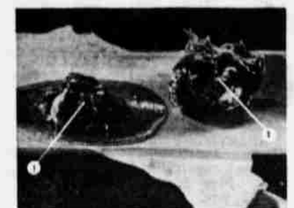
Blowtorch heats premium soap-base grease at left and Shell Darina AX at right. Soap-base grease slumps and liquefies (1), but Shell Darina AX (2) does not melt; it stays thick and buttery.
