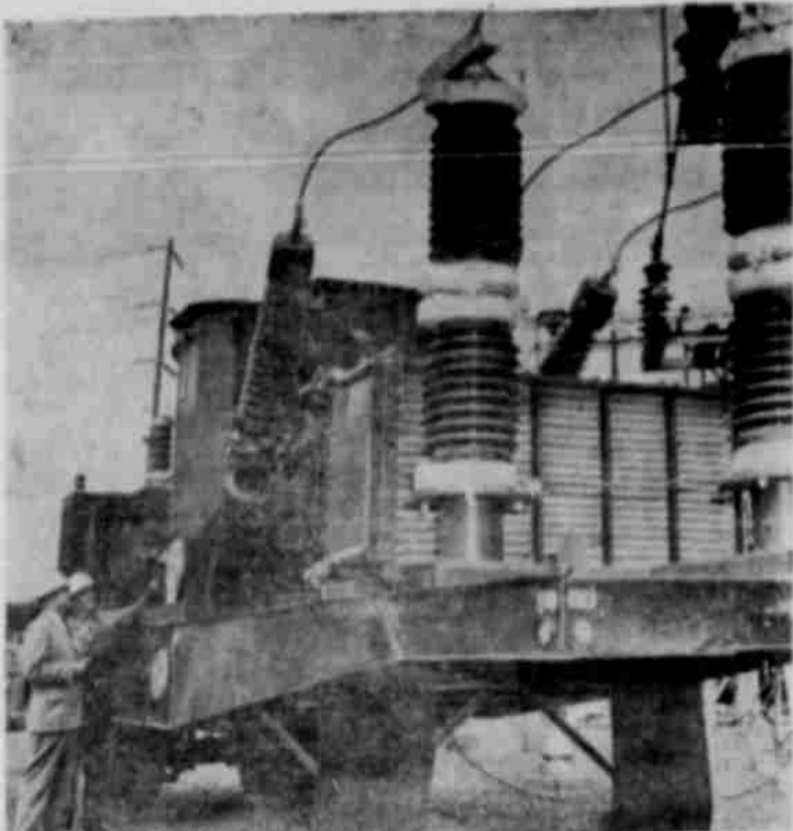
MOBILE MONSTER READY TO ROLL —Massive bushings of 50,000 pound trailer-mounted transformer give this newest Pacific Power & Light Company emergency-service unit a futuristic shape. PP&L has two of the monsters strategically located on its system, ready to roll over Oregon highways when needed at company substations to maintain electric service to customers.
