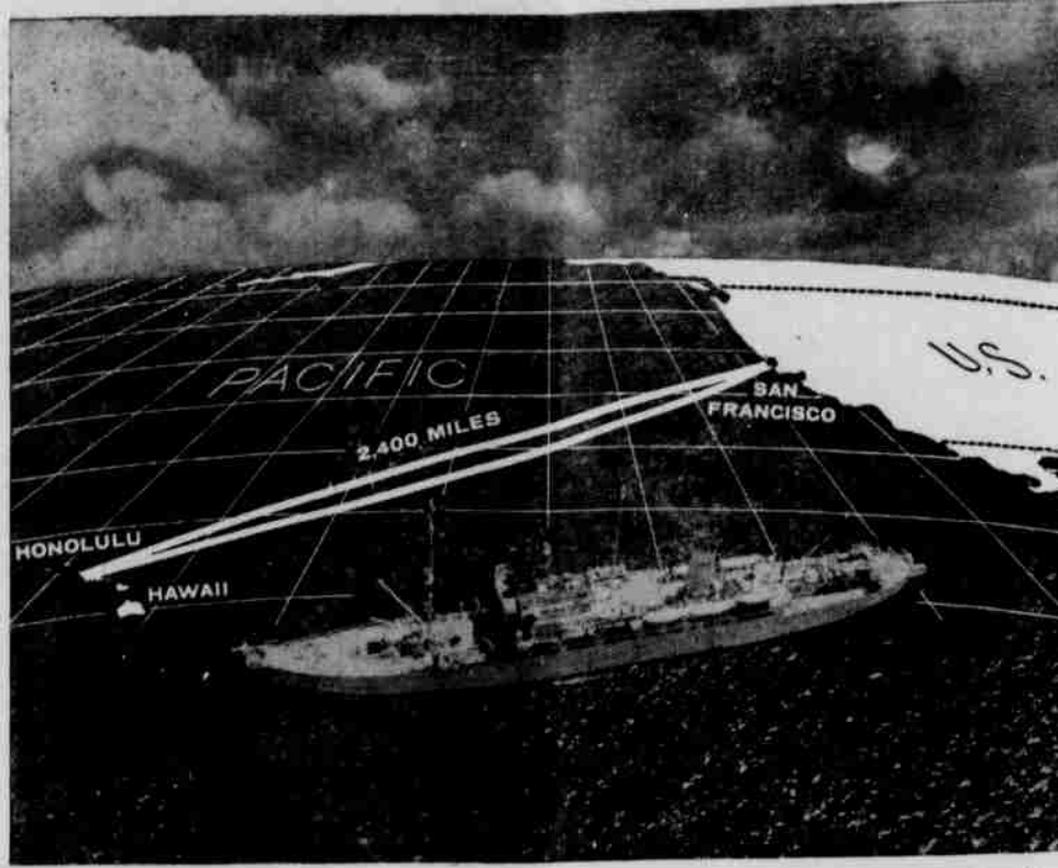
THE HMTS MONARCH, world's largest cables ship teamed with another vessel to lay the two telephone cables between Hawaii and the mainland during July, August and September. The new cable system, now in service, is the world's longest and deepest underwater telephone cable system.
