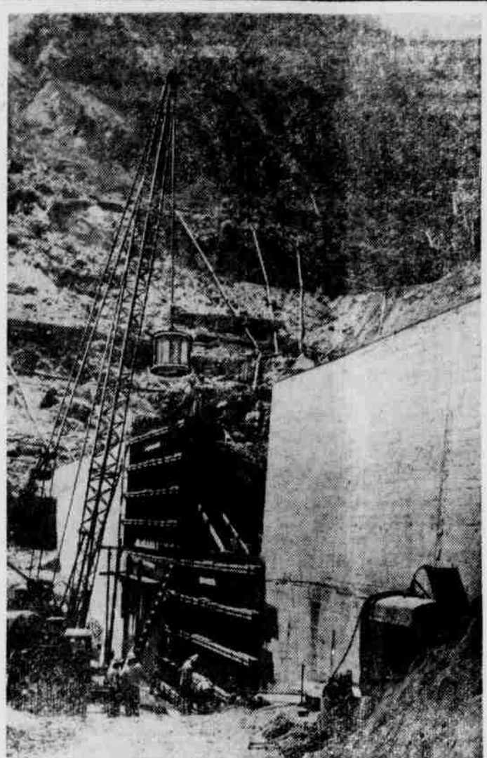
PROJECT MILESTONE — Completion of foundation work for Pacific Power & Light Company's Swift hydroelectric project marks another advance for the $51,000,000 development on the Lewis River. Section of 30-foot high, 300-foot long concrete wall, shown above, is portion of cut-off designed to prevent seepage beneath what will become world's highest earth-fill hydroelectric dam. The wall is being buried under millions of tons of rolled earth.
