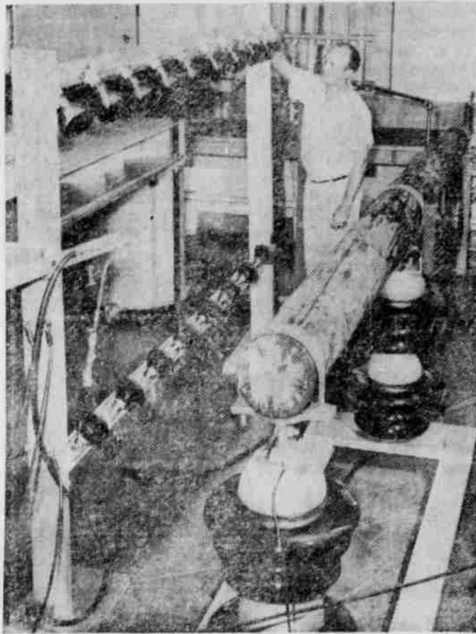
OREGON STATE COLLEGE—The problem of cross arm burning on high voltage power lines has been taken "indoors" for solution at Oregon State college's high voltage laboratory. There, electrical engineers are reproducing outdoor weather conditions in tests on the fir cross arm poles by means of sun lamps, a fog nozzle that gives fog and rain, and lines carrying 110,000 volts. The costly burning occurs early in the fall when insulators on the cross arms have been coated with dust or salt spray, allowing power leaks to short into the cross arm and char them. Don Hill, electrical engineering senior from Pendleton, shown here in the laboratory, is assisting Professor Louis N. Stone on the project. Eliminating the problem would save thousands of dollars annually for power companies.
