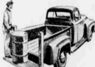
Hydraulic tailgate lifts 1,000 lbs., simplifies handling heavy items. Operates from single control at tailgate. Uses engine-mounted gear type hydraulic pump.
