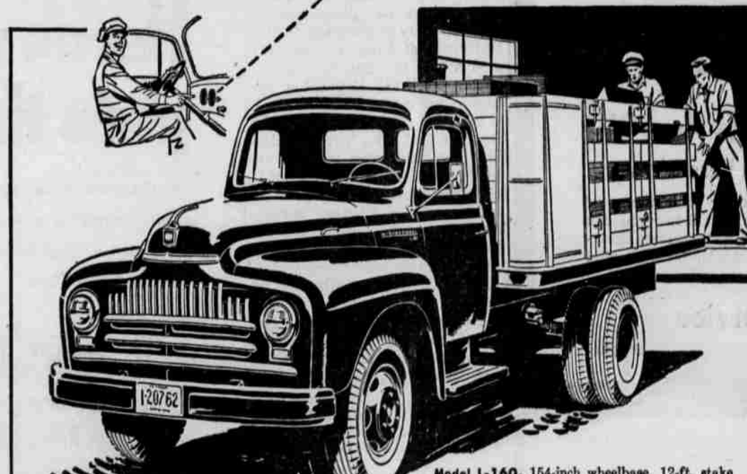
Model L-160, 154-inch wheelbase, 12-ft. stake body, 14,000 pounds GVW, featuring: Comfo-Vision Cab, "roomiest on the road," Silver Diamond 240 engine; 4-speed transmission. Specifications subject to change without notice.
