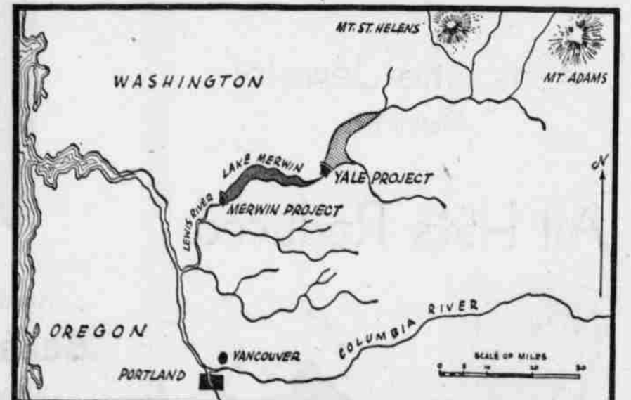
YALE SITE is immediately above the Company's 100,000-kilowatt Merwin development on the Lewis River, about 40 miles north of Portland. Both plants benefit from heavy winter rainfall. Output of the new plant will flow through interconnected transmission systems, to bolster service throughout the Pacific Northwest.
