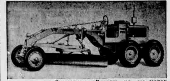
NEW 45 H.P. "CATERPILLAR" DIESEL NO. 212 MOTOR GRADER which has been announced in production by Caterpillar Tractor Co. The machine is powered by the new "Caterpillar" Diesel D311 Engine which also serves as the power source for the new, more powerful "Caterpillar" Diesel D2 track-type tractor. BRADEN TRACTOR & EQUIPMENT CO. Your JOHN DEERE and CATERPILLAR Dealer
