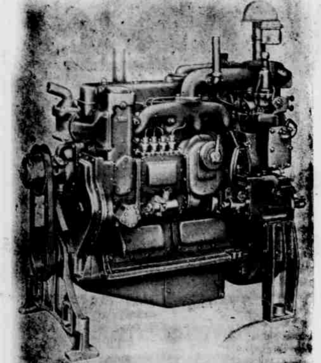
A NEW 4-IN. BORE ENGINE, THE "CATERPILLAR" DIESEL D311 engine, has been announced in production by Caterpillar Tractor Co. The engine, manufactured as an industrial power unit, electric set and marine engine, also is the power source for the new "Caterpillar" Diesel D2 track-type tractor and the "Caterpillar" Diesel No. 212 Motor Grader.
