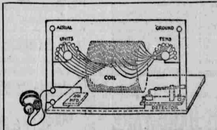
Diagram Showing How to Construct Simple Crystal Set That Gives Results
