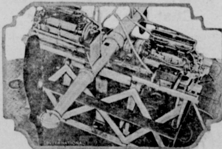
A view of the giant motors and the propellers of the new dirigible that is being built by a rubber company and is expected to take the place of the ill-fated "Roma," which exploded while on flight at Hampton Roads. The new dirigible is 170 feet long, of the non-rigid type, and has a capacity of 180,000 cubic feet in the compartments of the bag.
