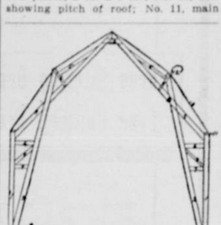
PLANK SYSTEM FRAME.
