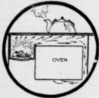
THE WIDE AND SHALLOW FIREBOX
