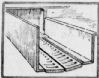
THE WIDE AND SHALLOW FIREBOX
