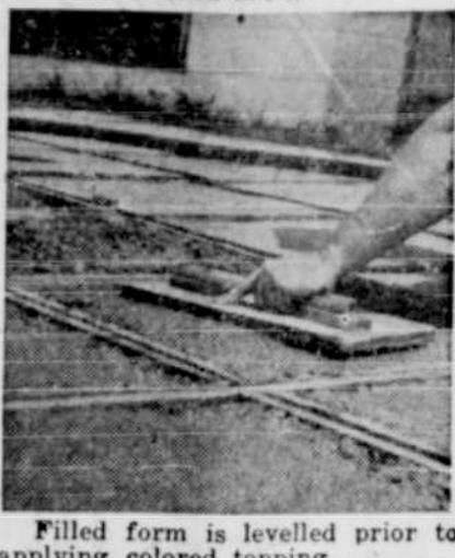
Filled form is levelled prior to applying colored topping.
