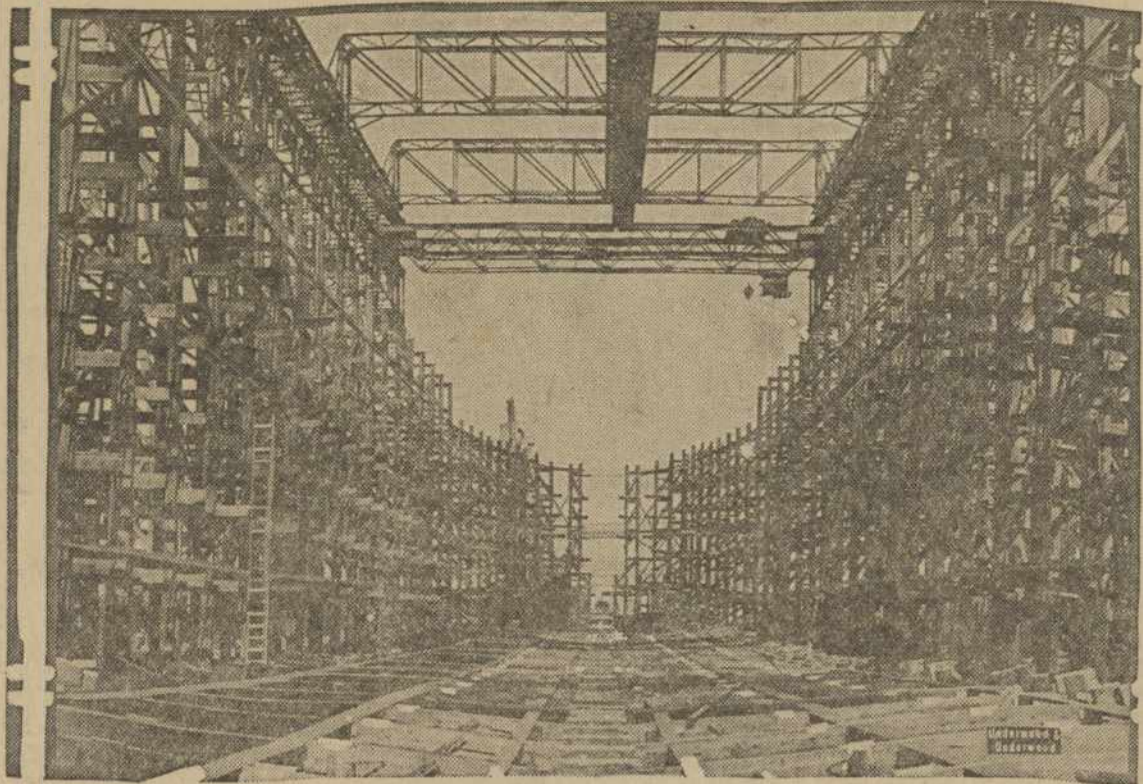
A new cruiser, the first since the Washington naval conference, is being built for the American navy at the Brooklyn navy yard. It will be called the Pensacola. The photograph shows the framework ready for the laying of the keel, which has just taken place.
