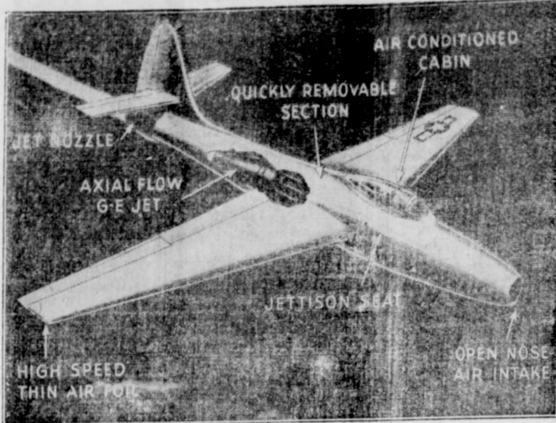
IT FLIES NEARLY 10 MILES A MINUTE—The Army Air Forces has just announced the new XP-84 fighter, powered by the new type axial flow G-E Jet, which will fly at a speed of 590 miles an hour and perform smoothly at well over seven miles above the earth. This schematic drawing of the Republic Thunderbolt shows in operation the axial flow jet engine, one of which was exhibited to the public for the first time at the General Electric Air Research Demonstration at the Schenectady Airport on June 21 and 22.
