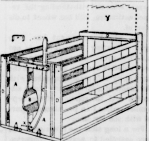
SIMPLE HOG-RINGING TRAP.
