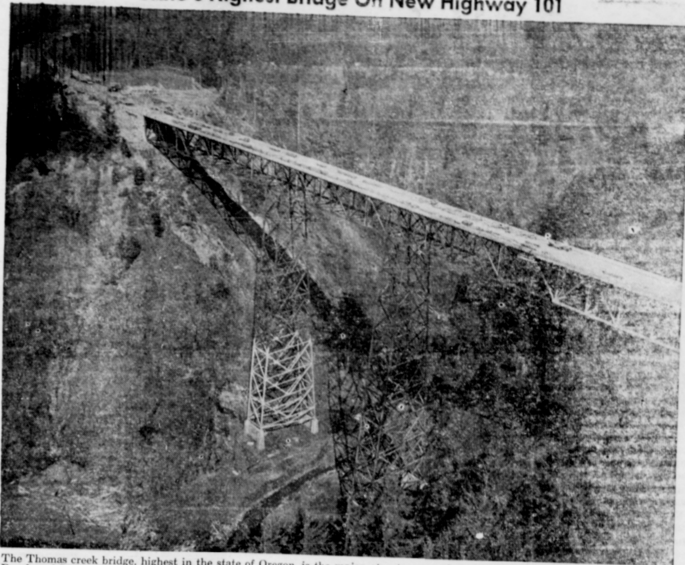
The Thomas creek bridge, highest in the state of Oregon, is the major structure on the relocated Highway 101 between Gold Beach and Brookings on the southern Oregon coast. The major section of the road will be dedicated and opened at the bridge site Dec. 9 by Oregon's Gov. Mark O. Hatfield. The bridge is 350 feet above the canyon floor and 957 feet long and cost $1,318,000. (Oregon State Highway Dept. Photo)
