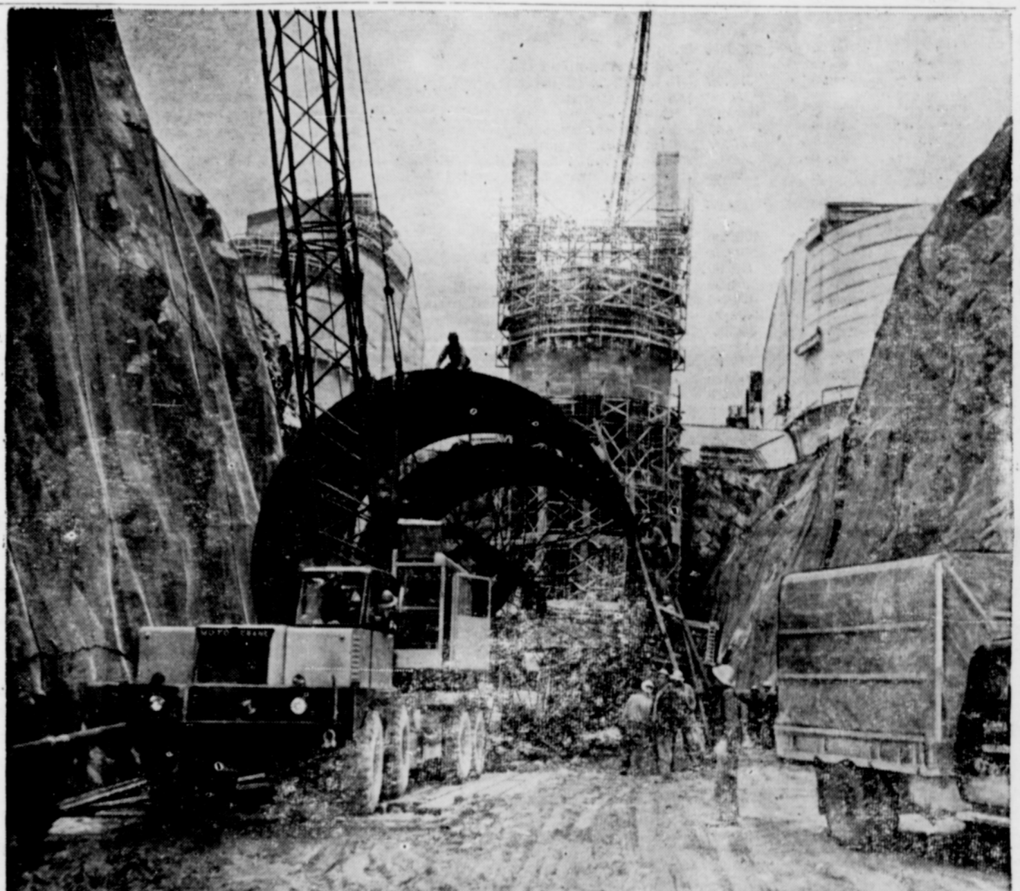
Twelve hundred men are on the job building the world's highest earth-fill dam at Pacific Power's huge Swift Hydroelectric Project on the Lewis River, one of the important new developments the Company now has under construction.
