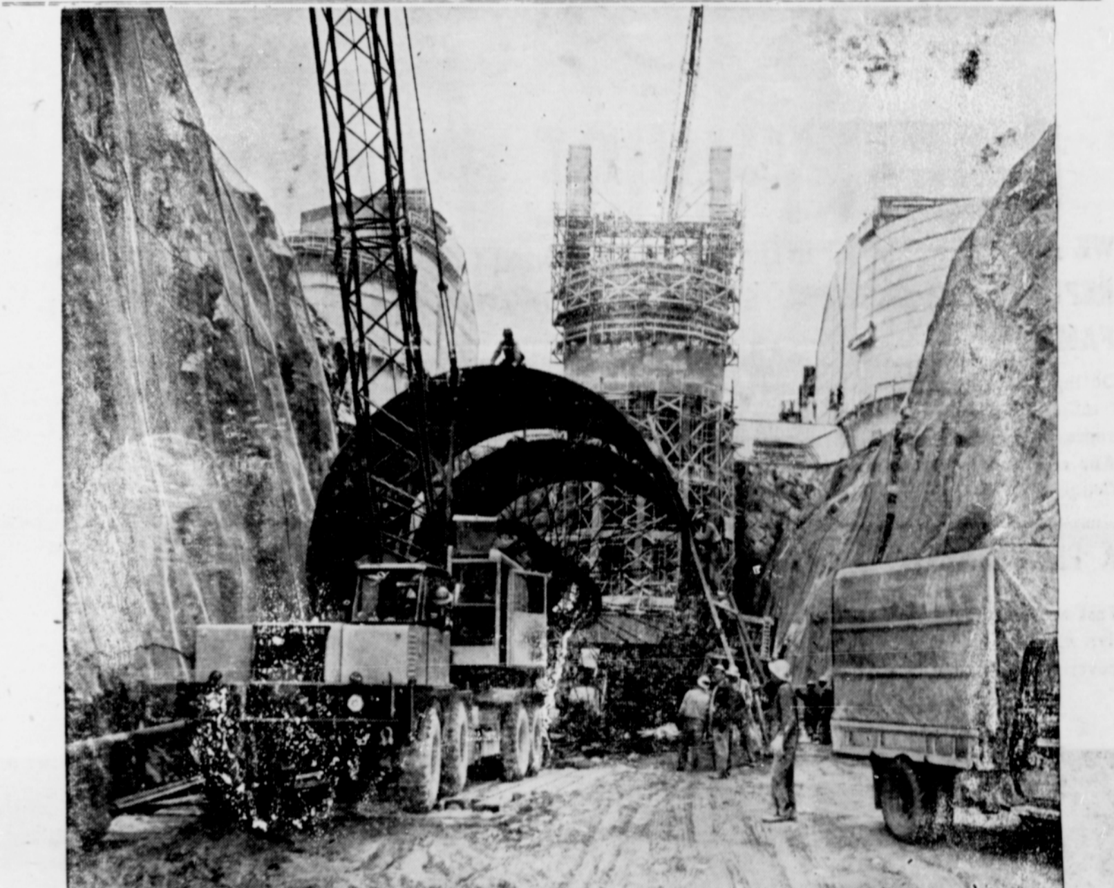
Twelve hundred men are on the job building the world's highest earth-fill dam at Pacific Power's huge Swift Hydroelectric Project on the Lewis River, one of the important new developments the Company now has under construction.
