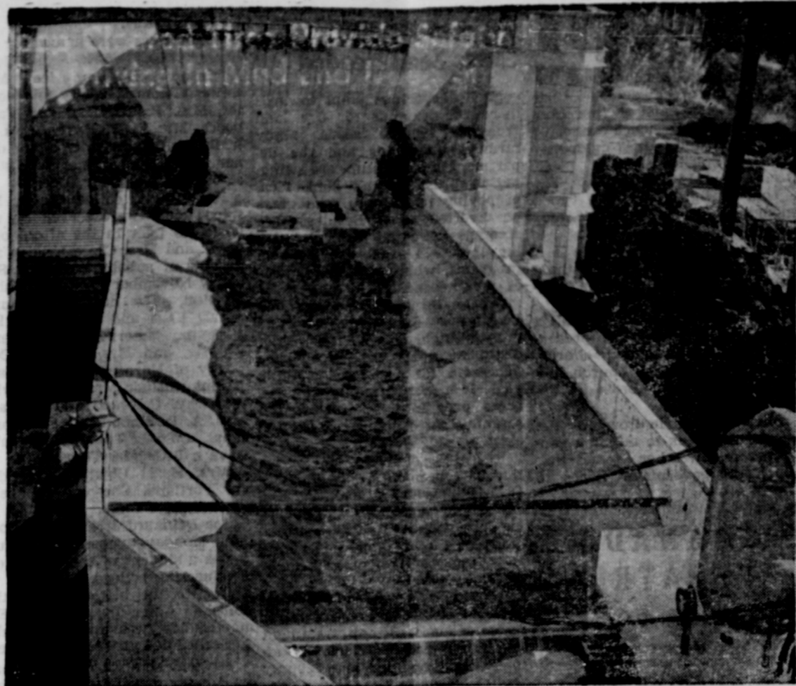
Pleasant Valley dam and topography of the Snake river canyon are reproduced to scale in this 64-foot long model of the proposed Pacific Northwest Power company power development just completed by the Washington State college division of industrial research. Under the direction of Dr. E. R. Tinney, WSC hydraulic engineer, right, workmen make adjustments on the 200-ton model as thousands of gallons of water thunder over the spillway as well as through powerhouse "turbines" to simulate actual over-flow and operating conditions.
