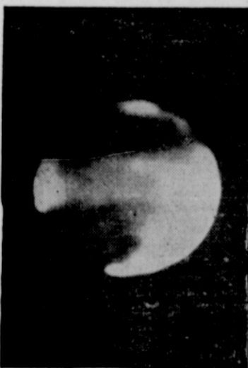
PLANET MARS . . . This photo shows permanent surface features of Mars. The large, dark areas were mapped by earliest visual observers and are well known.
